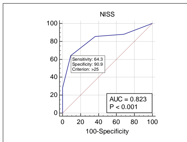
Figure [4]: ROC curve for NISS in prediction of HPCE.
